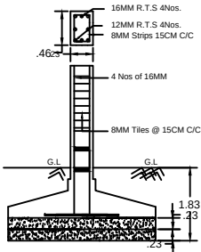
RCC COLUMN DETAILS
