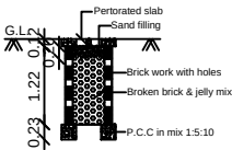
PERCOLATION PIT FOR 30 Sq. m. (Scale:- 1:50)
