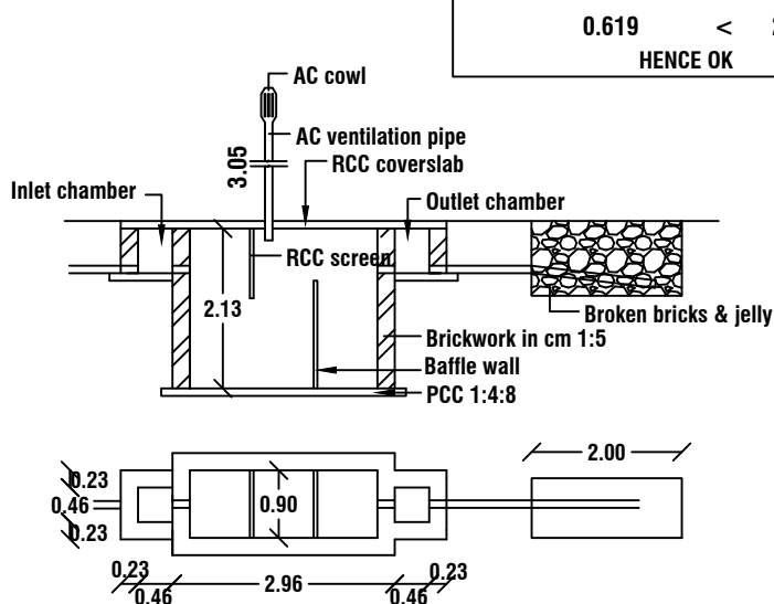
SEPTICTANK DETAILS
