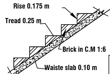
STAIR DETAILS
