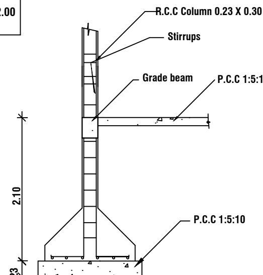
COLUMN DETAIL
