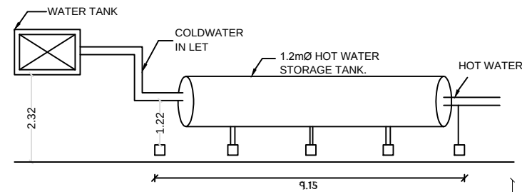
SOLAR WATER HEATING SWHS DETAIL
