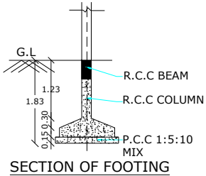
SECTION OF FOOTING
