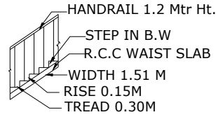
STAIR DETAIL
