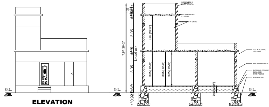
SECTION AA
