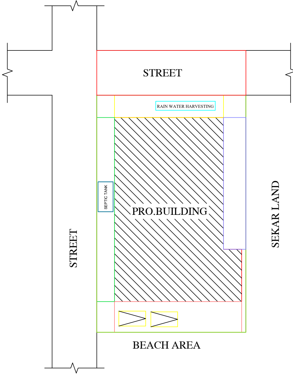
SITE PLAN
