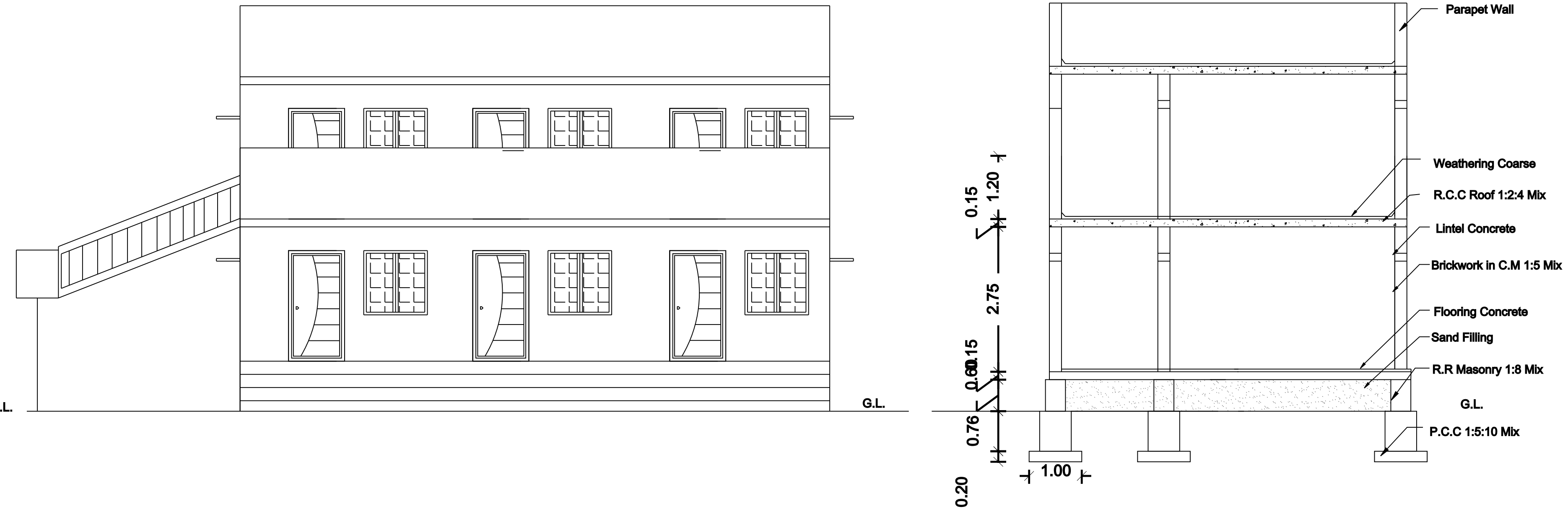
FRONT ELEVATION
