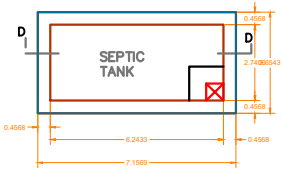
PLAN OF SEPTIC TANK SCALE 1"=2'-0"
