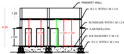
SECTION ON B-B
