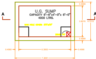
SUMP DETAIL
