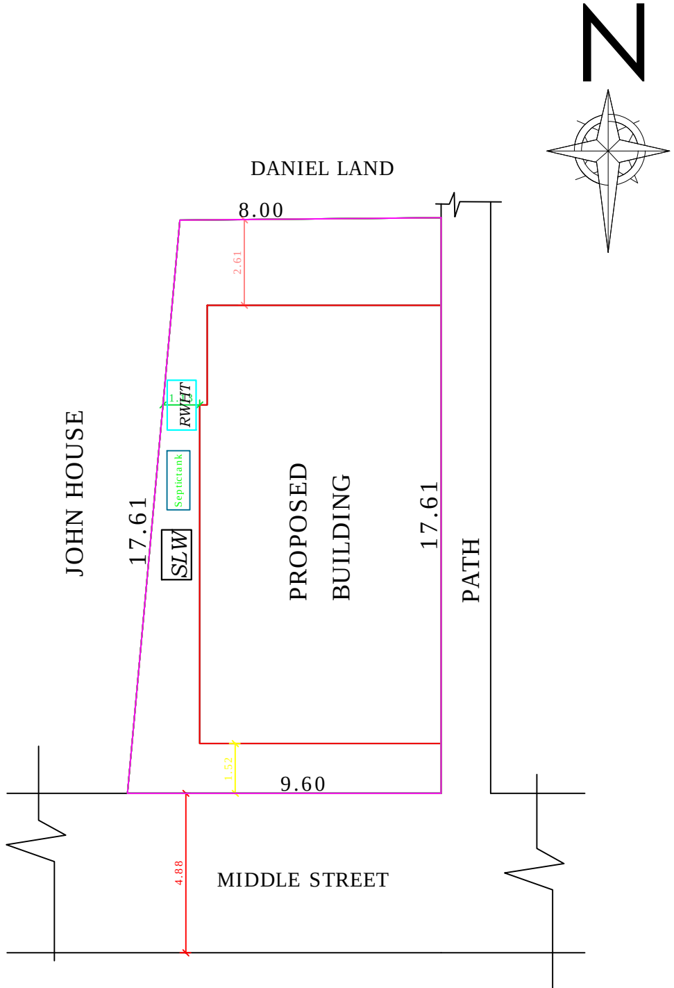
SITE PLAN
