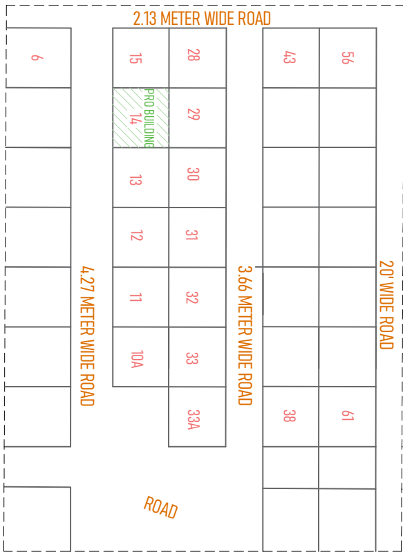
KEY PLAN
