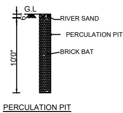
PERCULATION PIT
