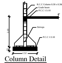
Column Detail
