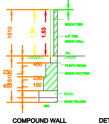
DETAIL
