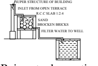
Rainwater harvesting
