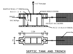
SEPTIC TANK AND TRENCH
