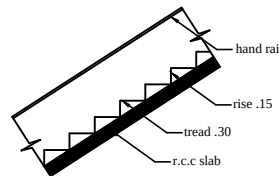
STAIR
