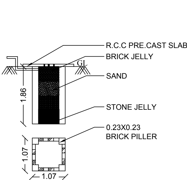
PLAN AND SECTION OF RAINWATER COLLECTION WELL
