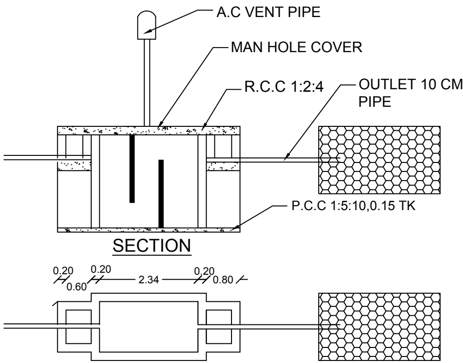
PLAN OF SEPTIC TANK & TRENCH
