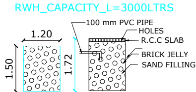
PLAN & SECTION OF RAIN WATER COLLECTION TANK
