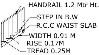
STAIR DETAIL
