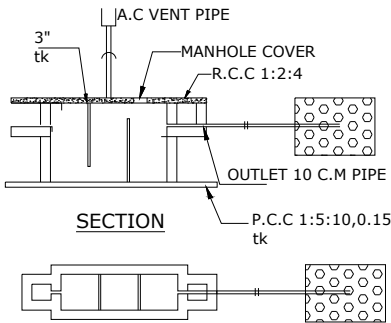
PLAN OF SEPTIC TANK & TRENCH
