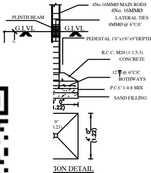
FOUNDATION DETAIL
