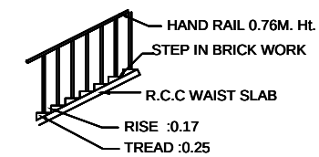
STAIR CASE DETAIL
