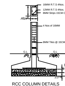
RCC COLUMN DETAILS
