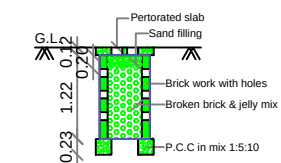
PERCOLATION PIT FOR 30 Sq. m. (Scale:- 1:50)
