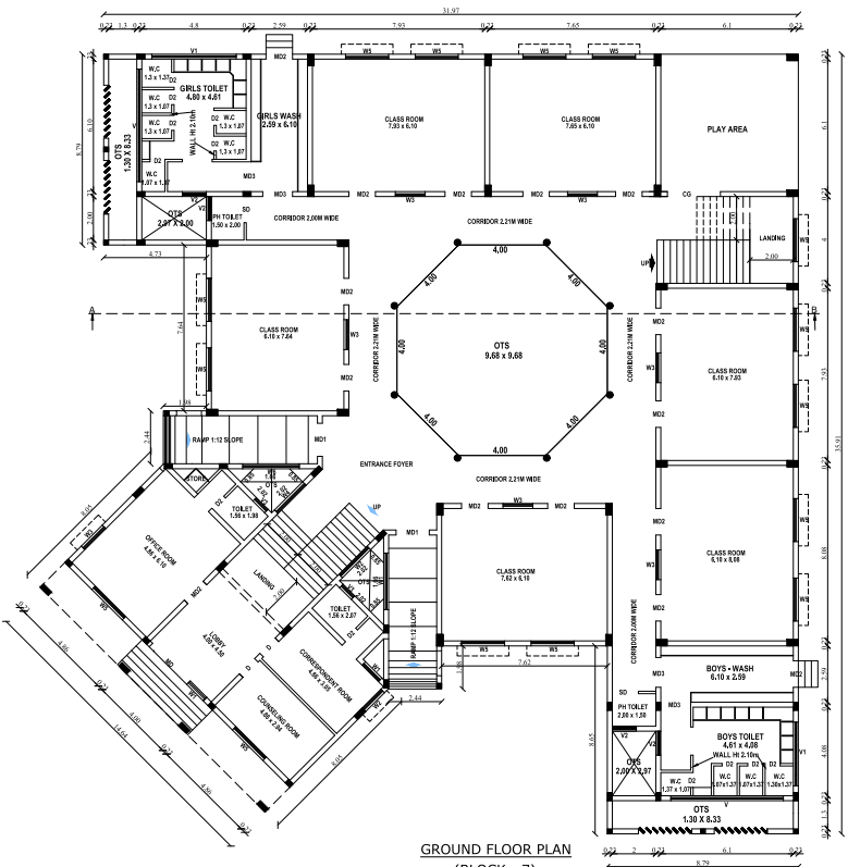
GROUND FLOOR PLAN (BLOCK - 7)
