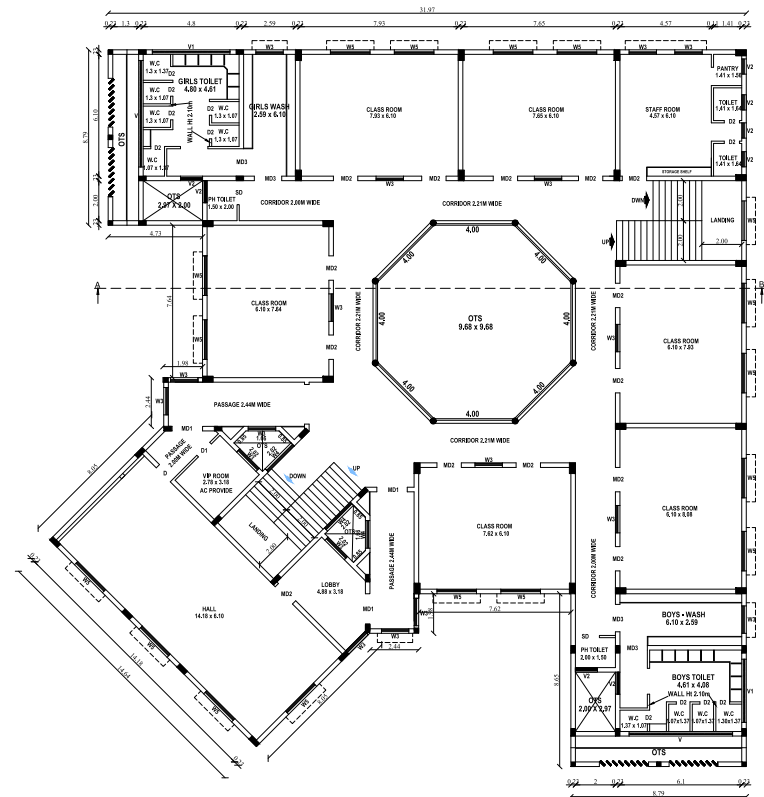
TYPICAL FIRST AND SECOND FLOOR PLAN
