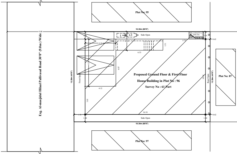
SITE PLAN
