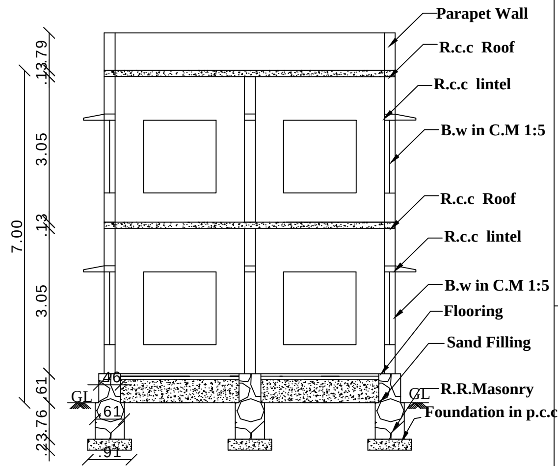
SECTION AB
