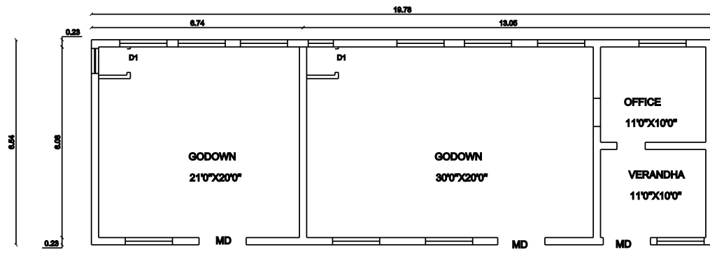
PLAN 1
