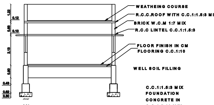
SECTION ON G1G2"
