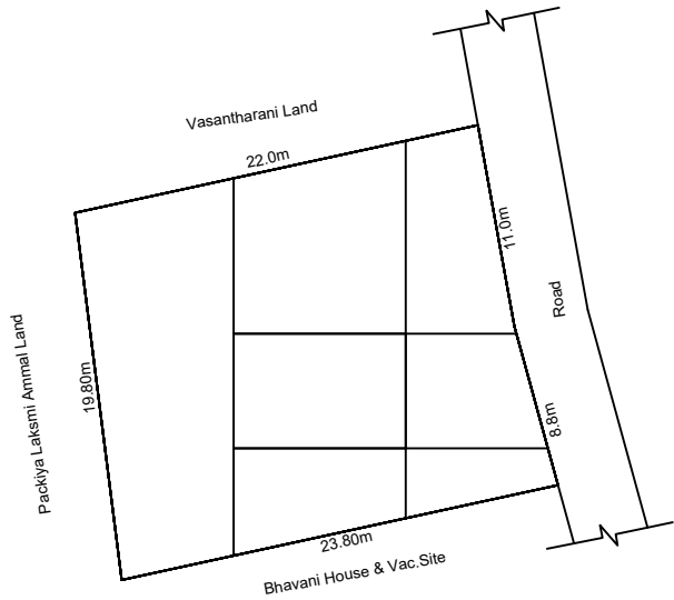
SITE PLAN
