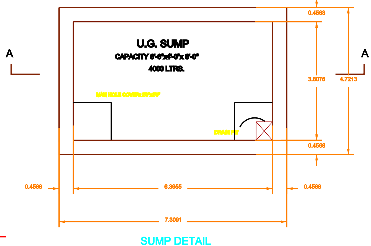
SUMP DETAIL
