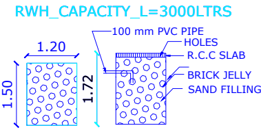
PLAN & SECTION OF RAIN WATER COLLECTION TANK
