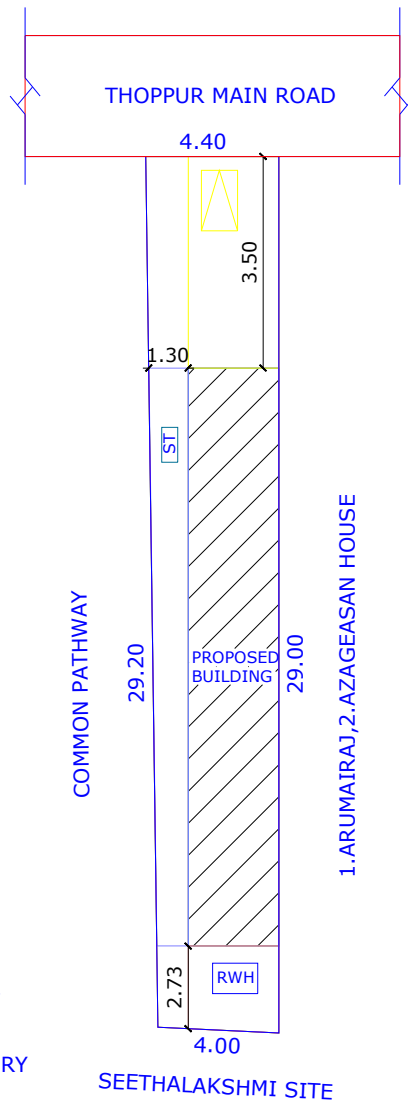
SITE PLAN
