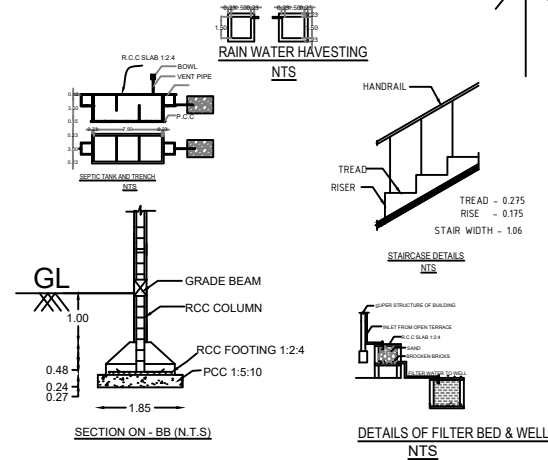
A.Kumaravel Chettiyar House & Vac.Site
