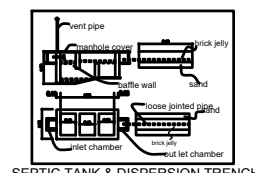
SEPTIC TANK & DISPERSION TRENCH
