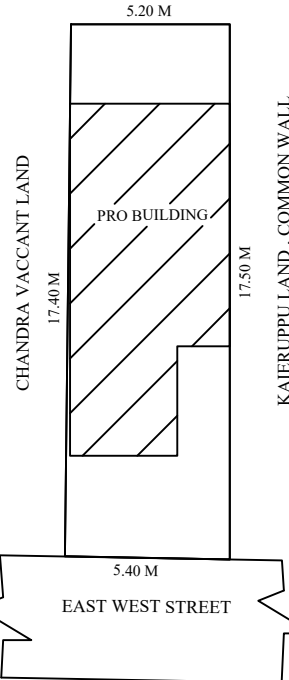
SITE PLAN
