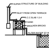
DETAILS OF FILTER BED & WELL NTS
