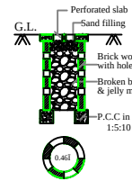
PERCOLATION PIT (NOT FOR SCALE)
