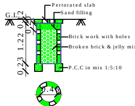
PERCOLATION PIT FOR 30 Sq. m. (Scale:- 1:50)
