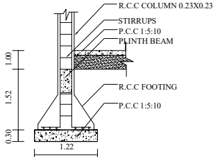
COLUMN DETAILS
