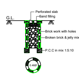
PERCOLATION PIT FOR 30 Sq. m.
