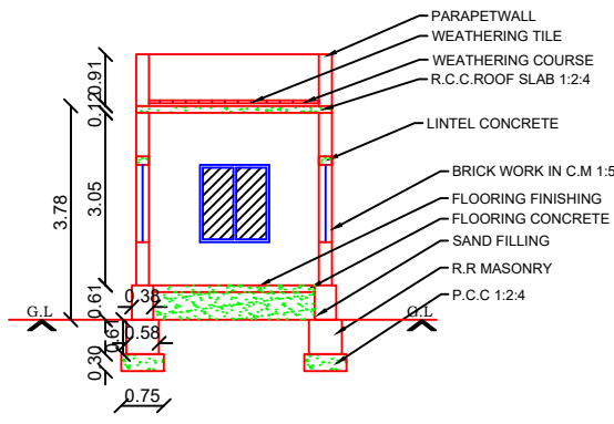
SECTION AT A-B
