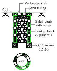
PERCOLATION PIT (NOT FOR SCALE)
