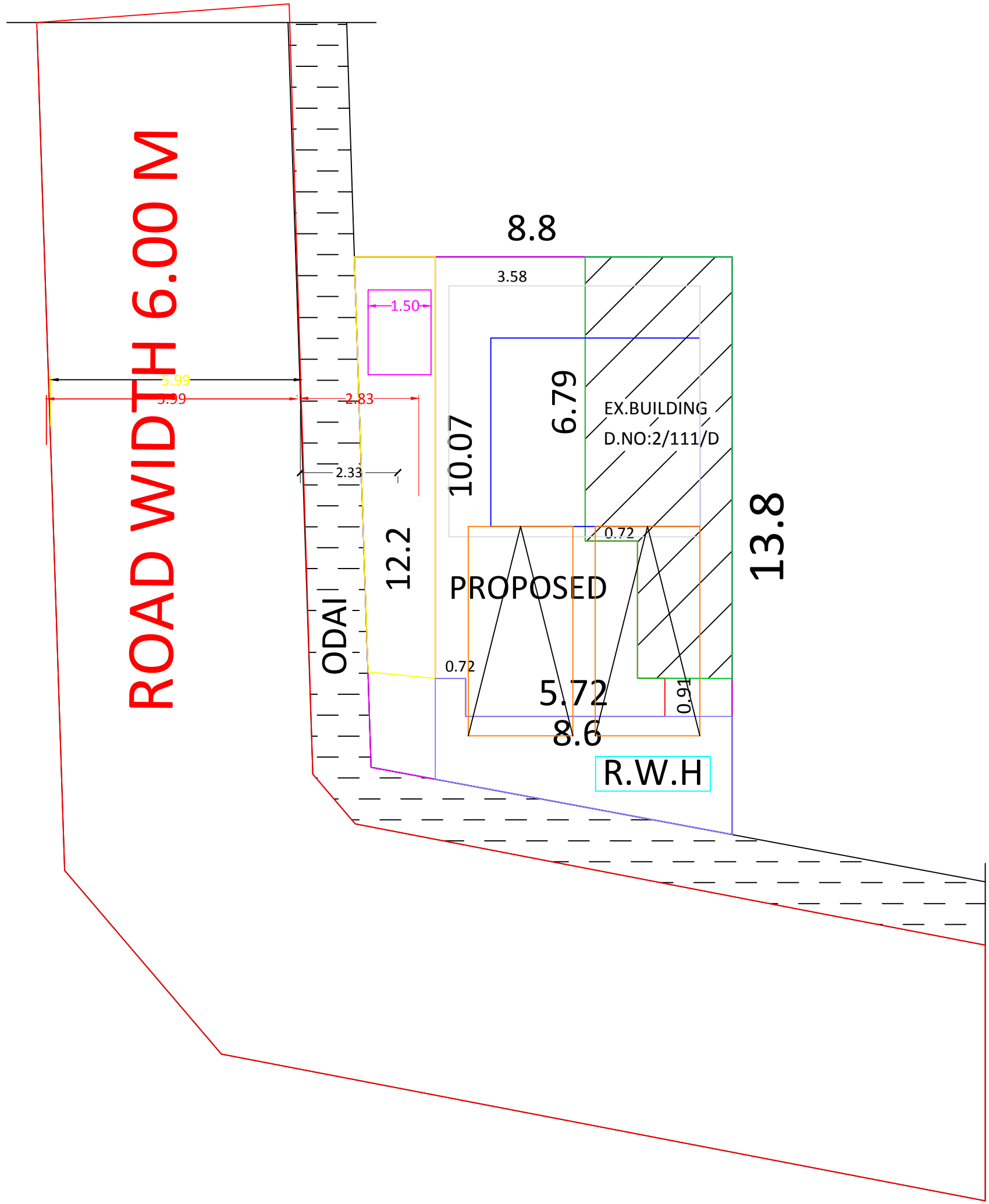
SITE PLAN
