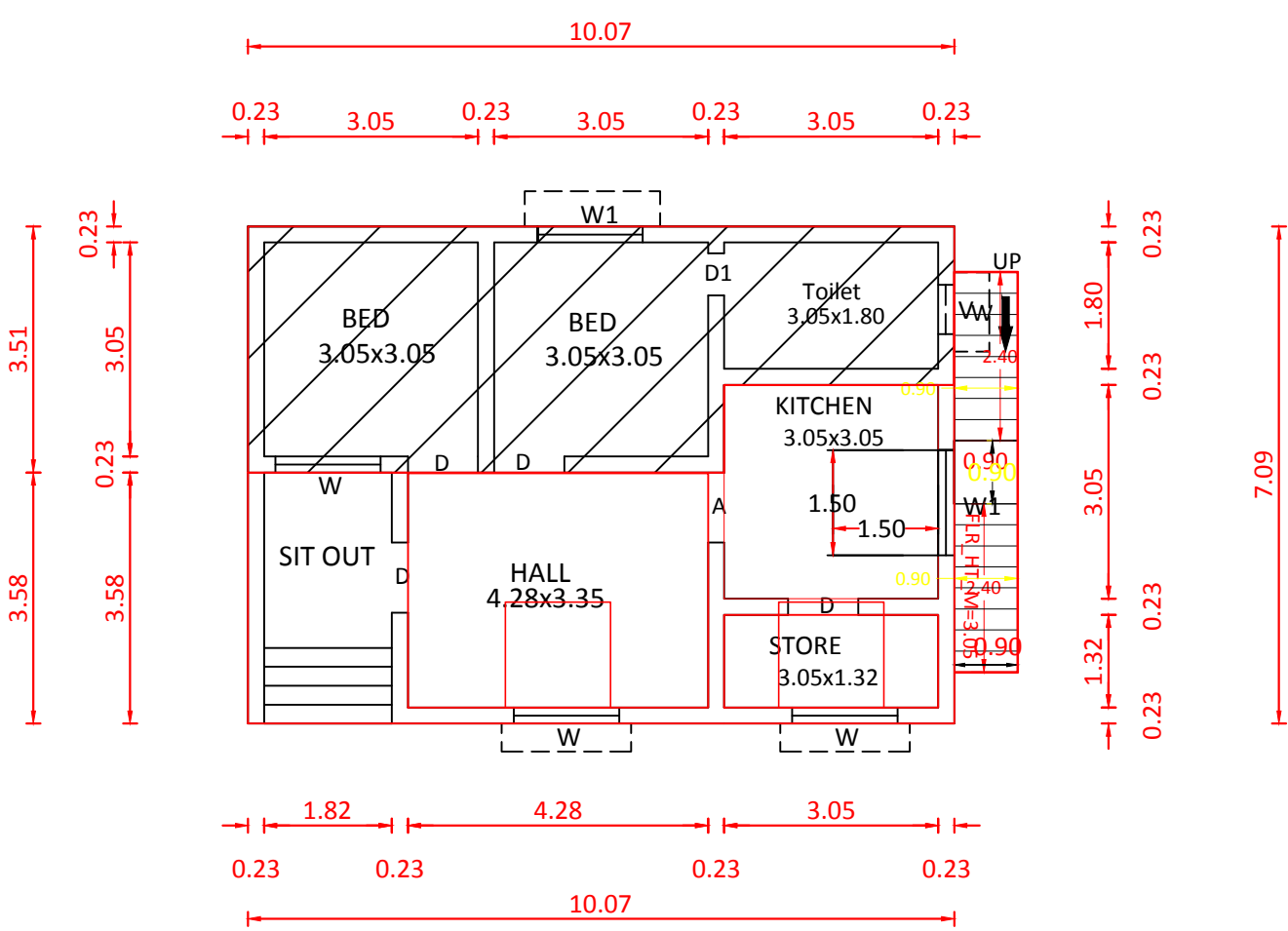
EX.GROUND FLOOR PLAN & PRO.GROUND FLOOR PLAN
