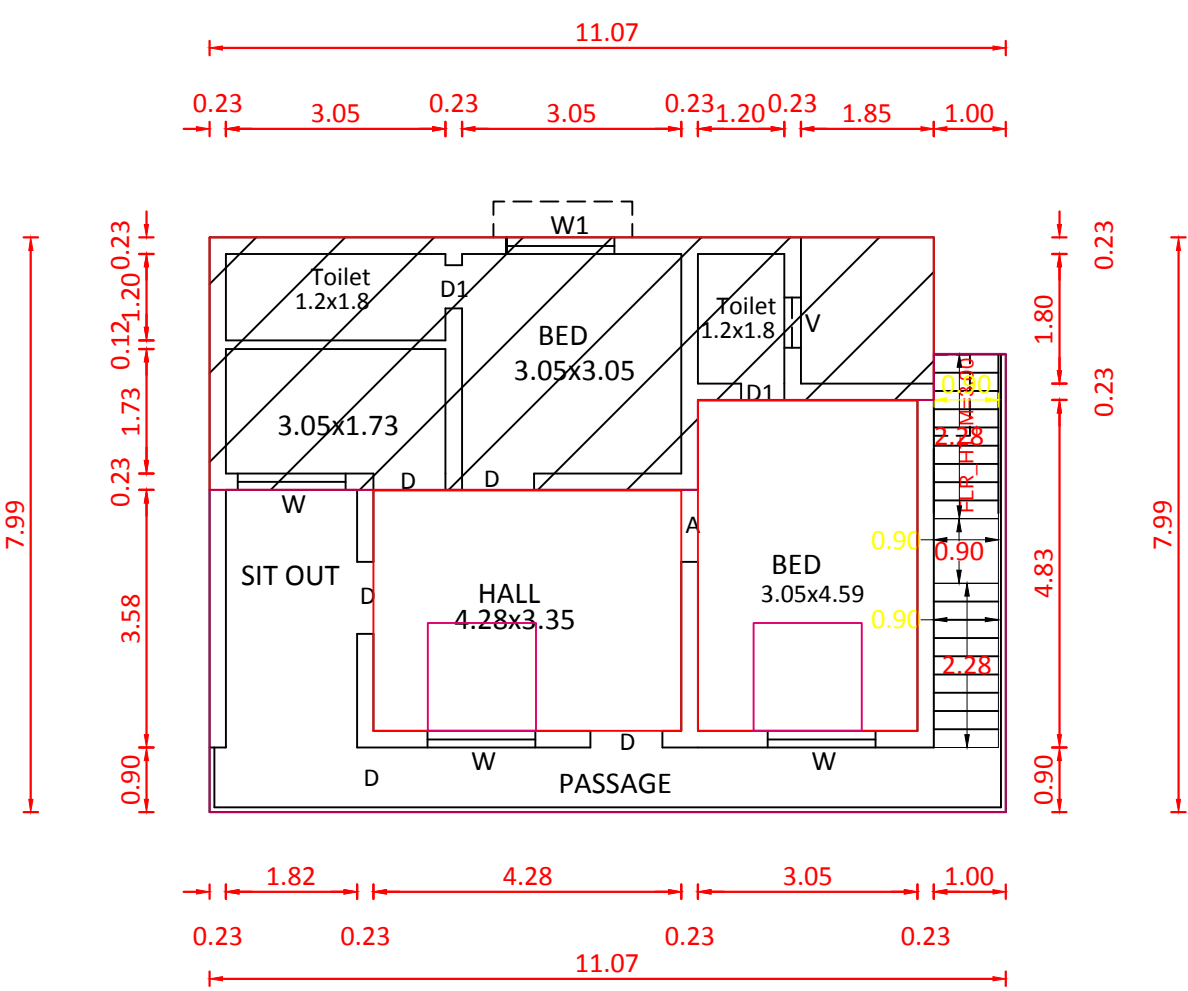
EX.FIRST FLOOR PLAN & PRO.FIRST FLOOR PLAN
