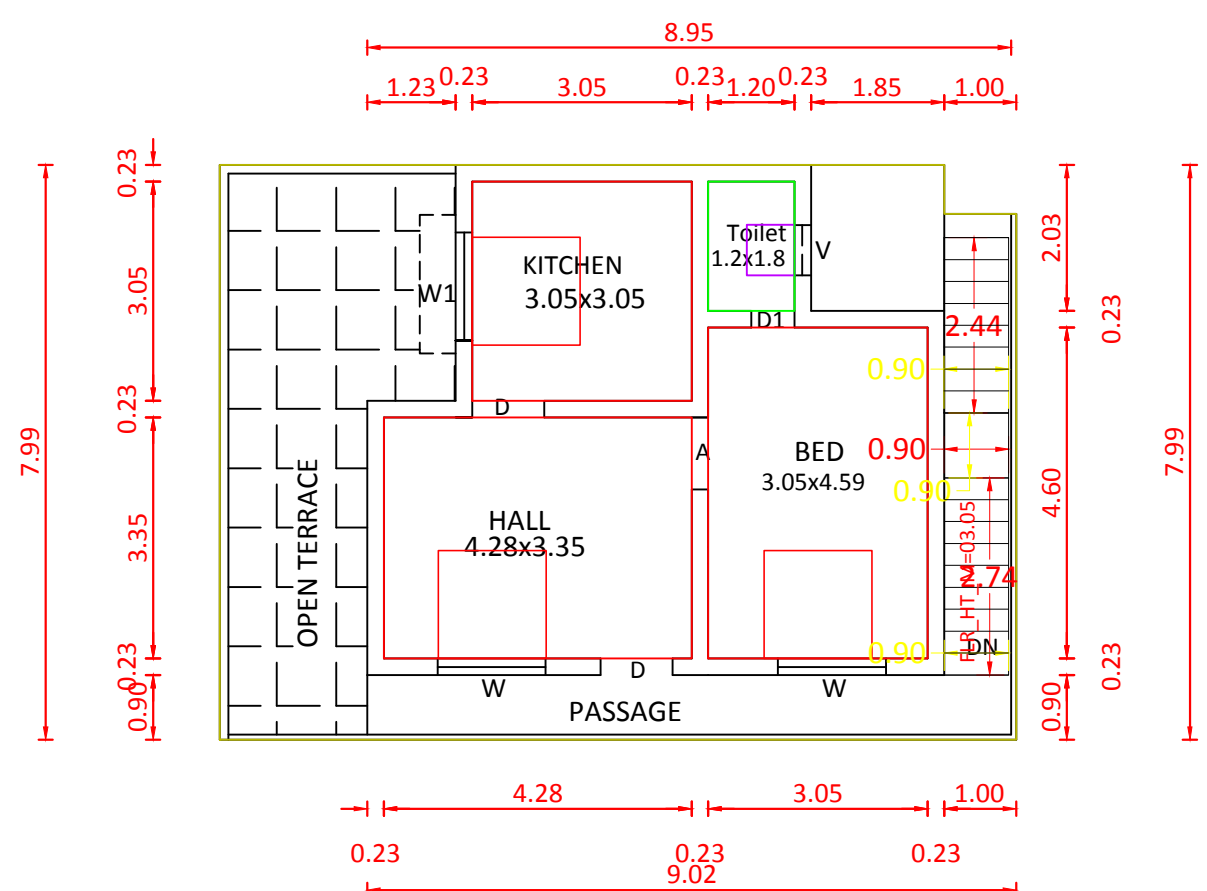
PRO.SECOND FLOOR PLAN
