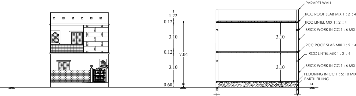
SECTION ON AB &( HALF ELEVATION)
