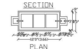
SEPTIC TANK DETAILS
