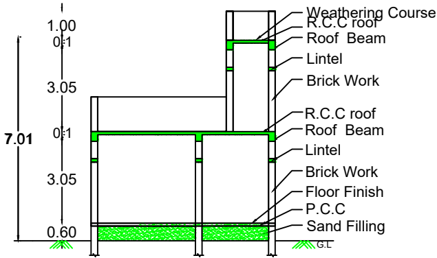
SECTION AB
