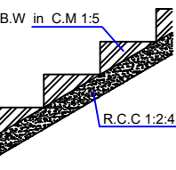
STAIRCASE
