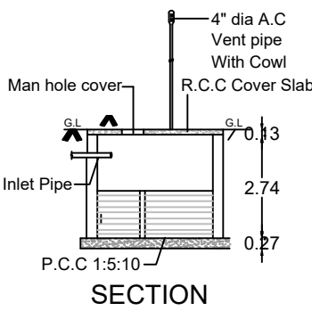
SECTION OF RECHARGE TRENCH METHOD
