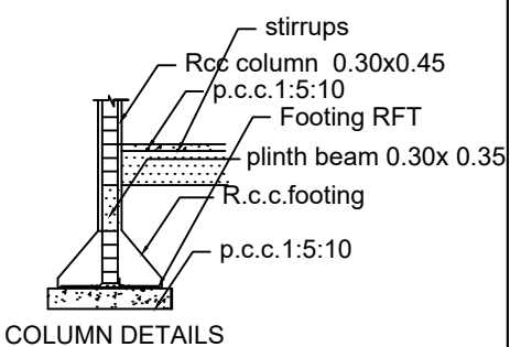
COLUMN DETAILS
