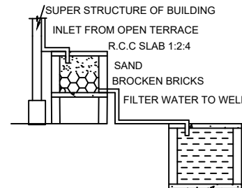
RAINWATER HARVESTING
