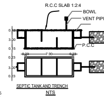
SEPTIC TANK AND TRENCH
