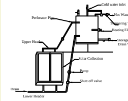
Details Of Solar Water Heater (NTS)
