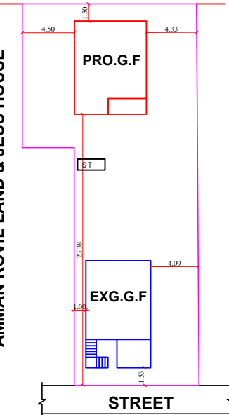
SITE PLAN SCALE 1:200
