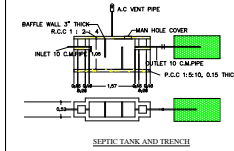
Septic Tank
