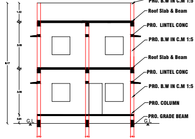
CROSS SECTION ON XX
