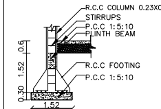
COLUMN DETAILS
