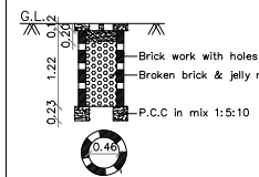
PERCOLATION PIT FOR 30 Sq. m. (Scale: - 1:50)
