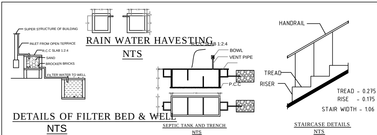
SEPTIC TANK AND TRENCH NTS
