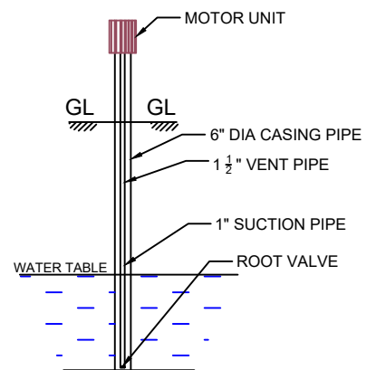
SEC.OF BOREWELL
