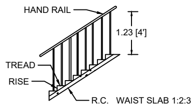
STAIRCASE DETAILS
