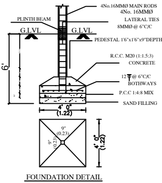
FOUNDATION DETAIL
