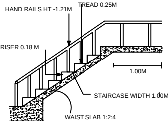
STAIRCASE DETAILS
