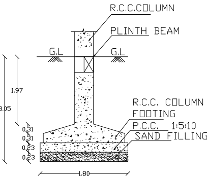
FOUNDATION DETAIL OFFICE USE
