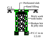
PERCOLATION PIT (NOT FOR SCALE)
