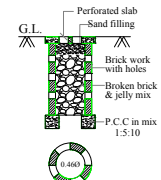
PERCOLATION PIT (NOT FOR SCALE)
