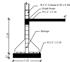
Column Detail
