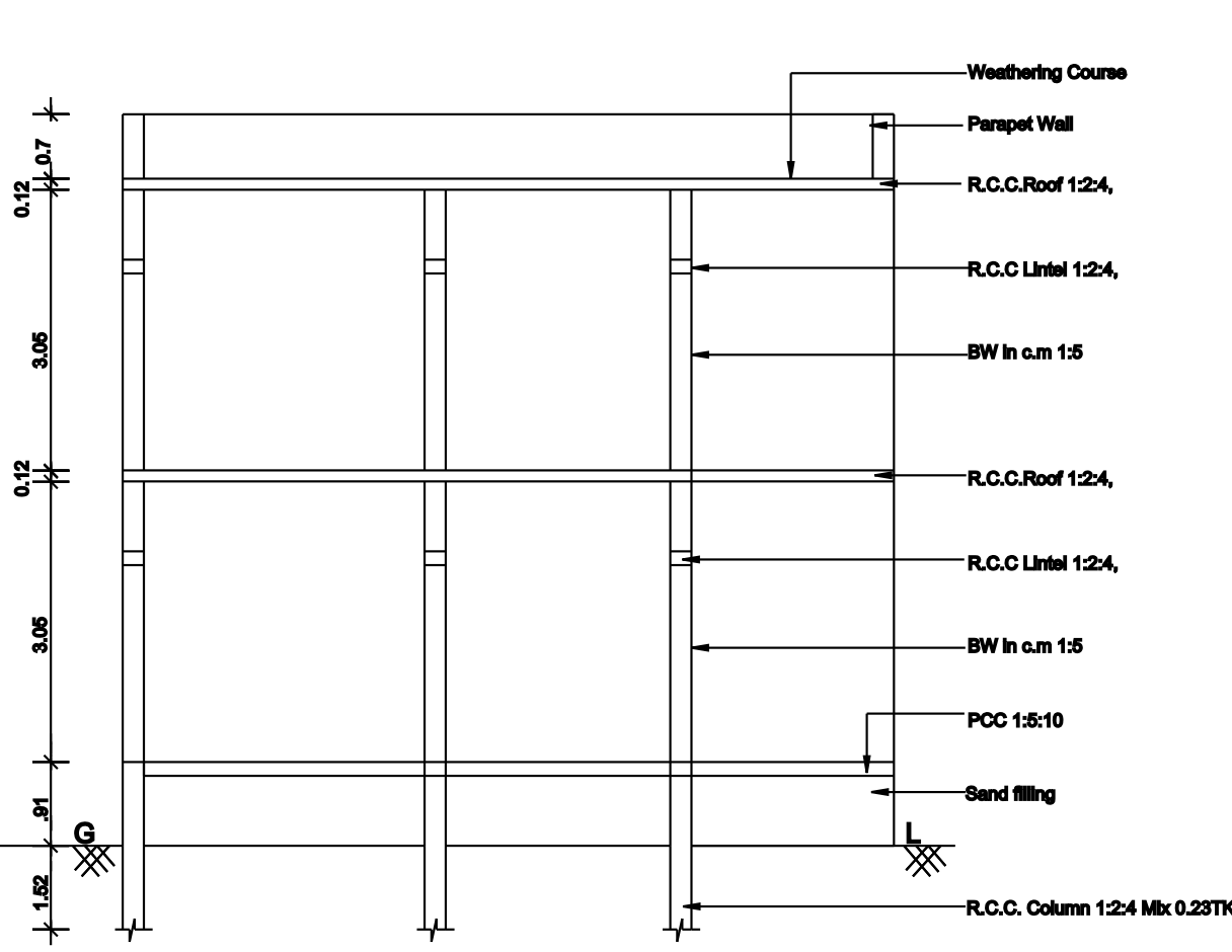
SECTION ON P-Q
