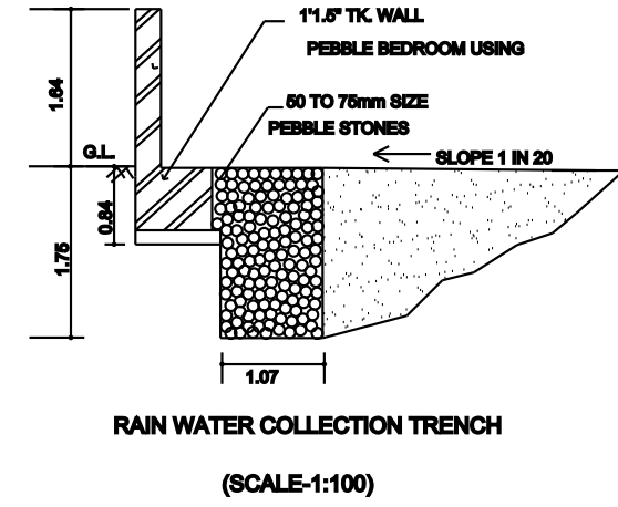
RAIN WATER COLLECTION TRENCH (SCALE:1:100)
