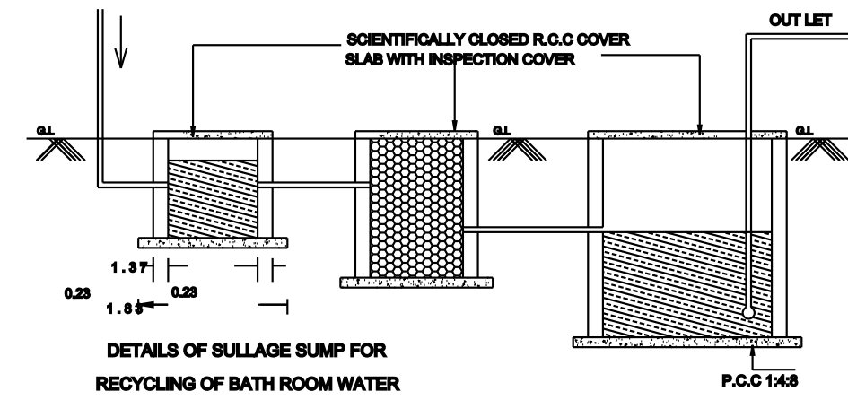
DETAILS OF BALLAGE PUMP FOR RECYCLING OF BATH ROOM WATER
