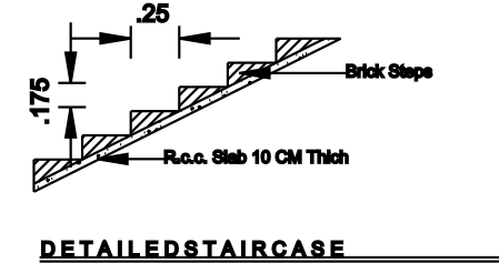
DETAILED STAIRCASE
