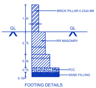
FOOTING DETAILS
